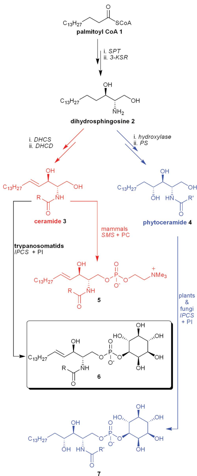
Fig. 1 Divergent pathways in phosphosphingolipid biosynthesis (SPT, serine palmitoyl transferase; 3-KSR, 3-ketosphinganine reductase; DHCS, dihydroceramide synthase; DHCD, dihydroceramide desaturase; PS, phytoceramide synthase; SMS sphingomyelin synthase; IPCS inositol ceramide synthase; PC phosphatidylcholine; PI phosphatidylinositol).
