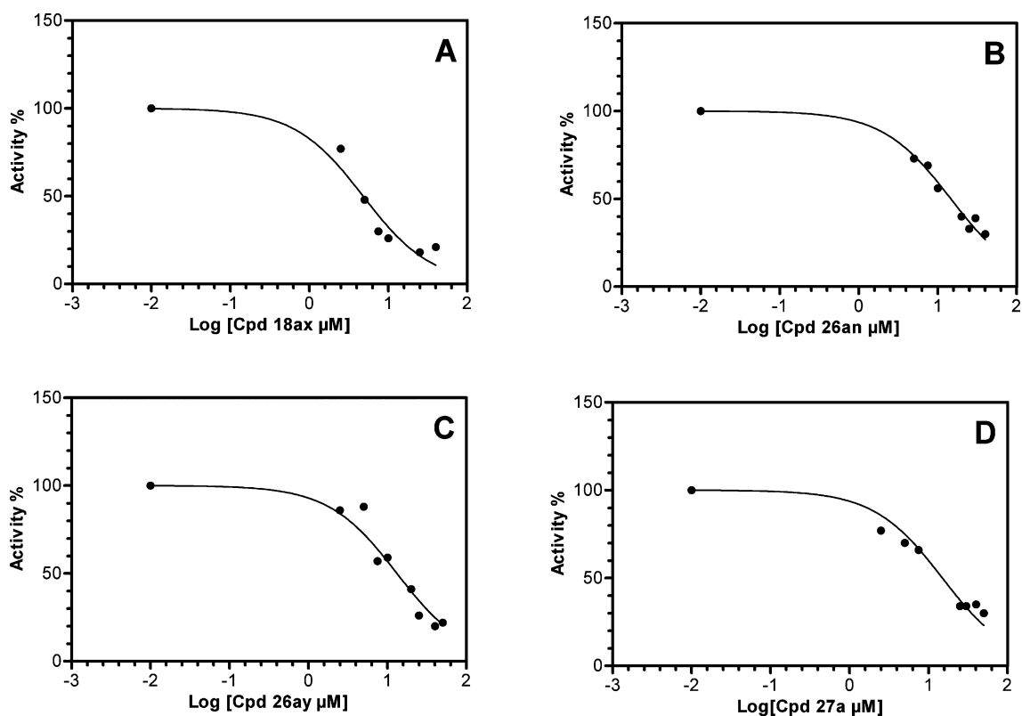
Fig. 4 Inhibition curves and IC_{50} values of selected inhibitors. Activity refers to percentage activity relative to untreated control. Calculated IC_{50} values A (18ax) 4.8 \mu M; B (26an) 14.7 \mu M; C (26ay) 13.2 \mu M; D (27a) 15.0 \mu M.
